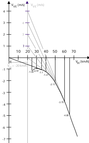
Illustration: polar with and without a head wind
