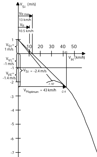
Illustration: Optimized desired flight
